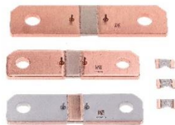
Current Sensing Resistors for Portable Devices / Automotive / Industrial Applications Small Sizes down to 0201\text{mm} High Wattage up to 36\text{W}
